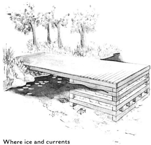
Where ice and currents permit, rock-filled cribs can make a solid dock foundation.
