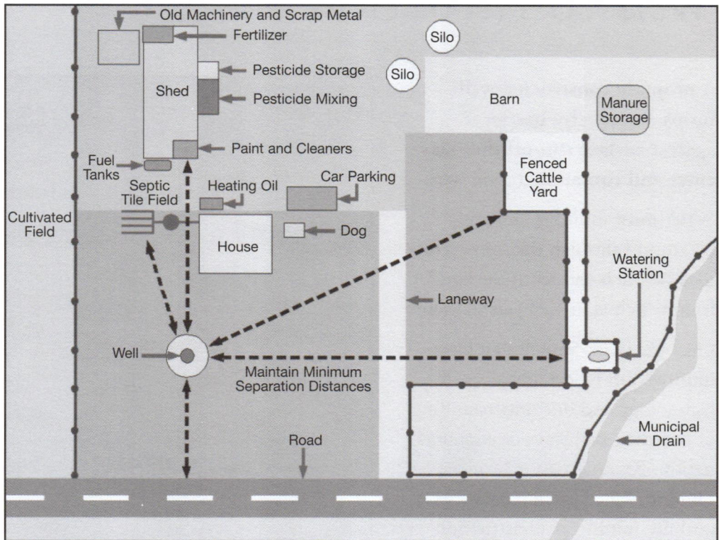
Verify adequate separation from potential contaminants. Credit: BMP: Water Wells
