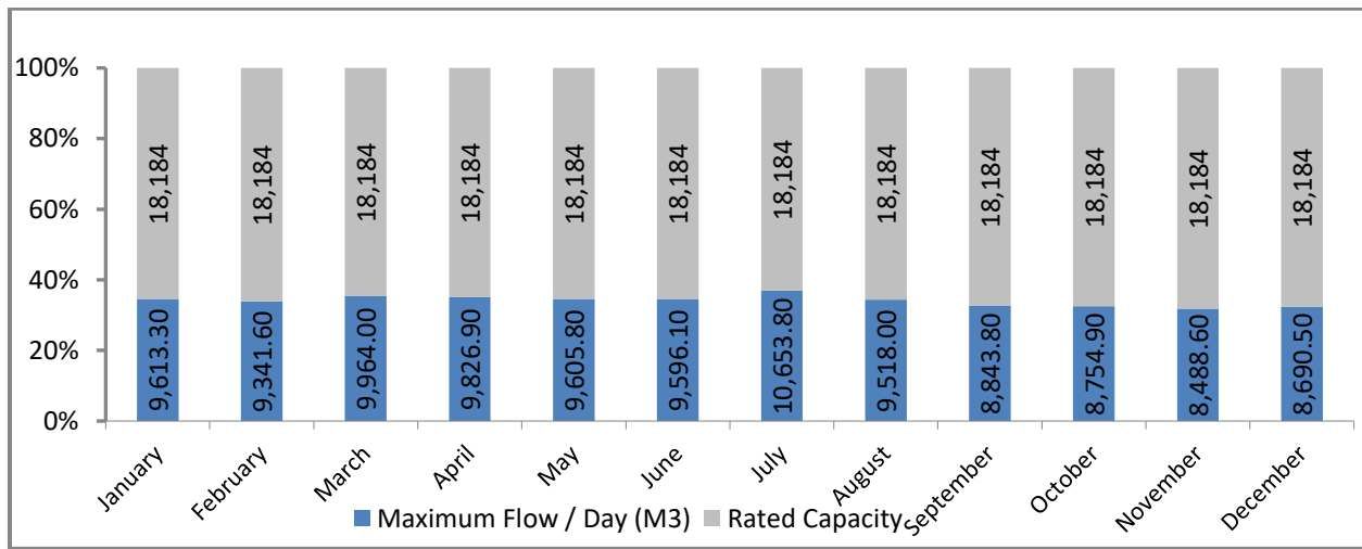
Comparison of Maximum Daily Flow to Rated Capacity 2022 for Raw Water
