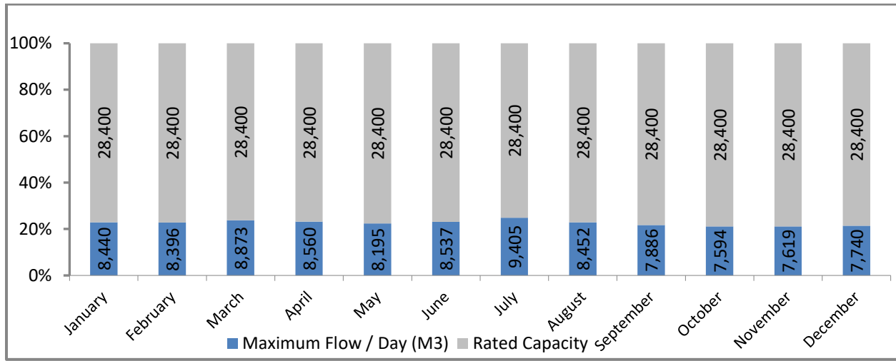
Comparison of Maximum Daily Flow to Rated Capacity 2022 for Treated Water
