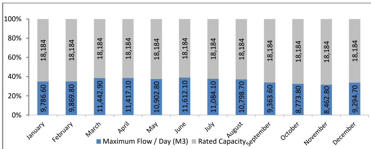
Comparison of Maximum Daily Flow to Rated Capacity 2021 for Raw Water
