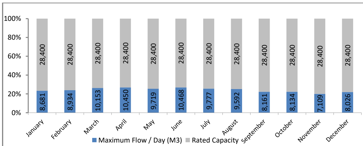
Comparison of Maximum Daily Flow to Rated Capacity 2021 for Treated Water
